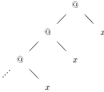
Fig. 1. A paradoxical infinite term
