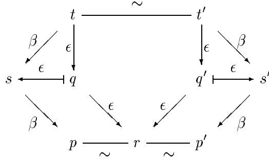
Fig. 9. Theorem 57: the Church-Rosser property, up to equivalence
